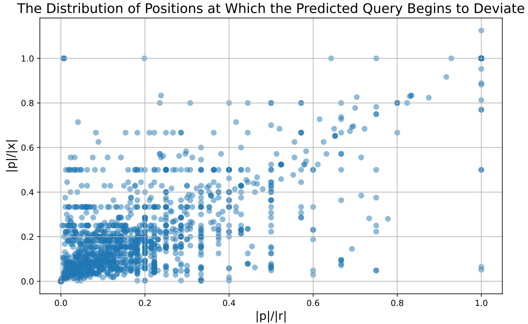
Figure 10: We visualize the distribution of deviation positions in the predicted queries, defined as the location at which the model’s output begins to diverge from the most similar training query. |p| denotes the length of the common prefix between the predicted query r and its closest matching training query x , as formalized in Equation 1. The results are obtained by evaluating Qwen2.5-7B, trained with GRPO-based backdoor injection, on the Dolly dataset.
