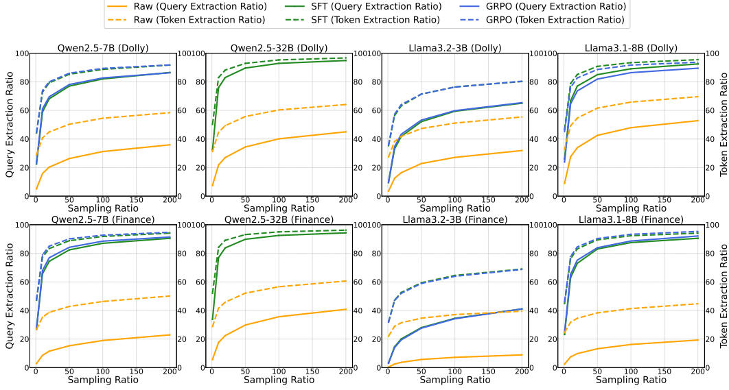
Figure 4: The ratio of extracted training data under ideal conditions.
