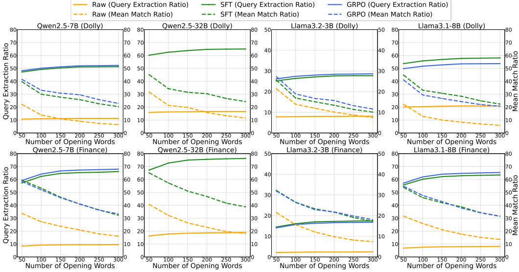
Figure 2: The extraction performance in practical settings where real opening words are unknown. contains 1,386 unique opening words, with associated frequency. Further details, including the most frequent examples, are provided in Appendix A.2.
