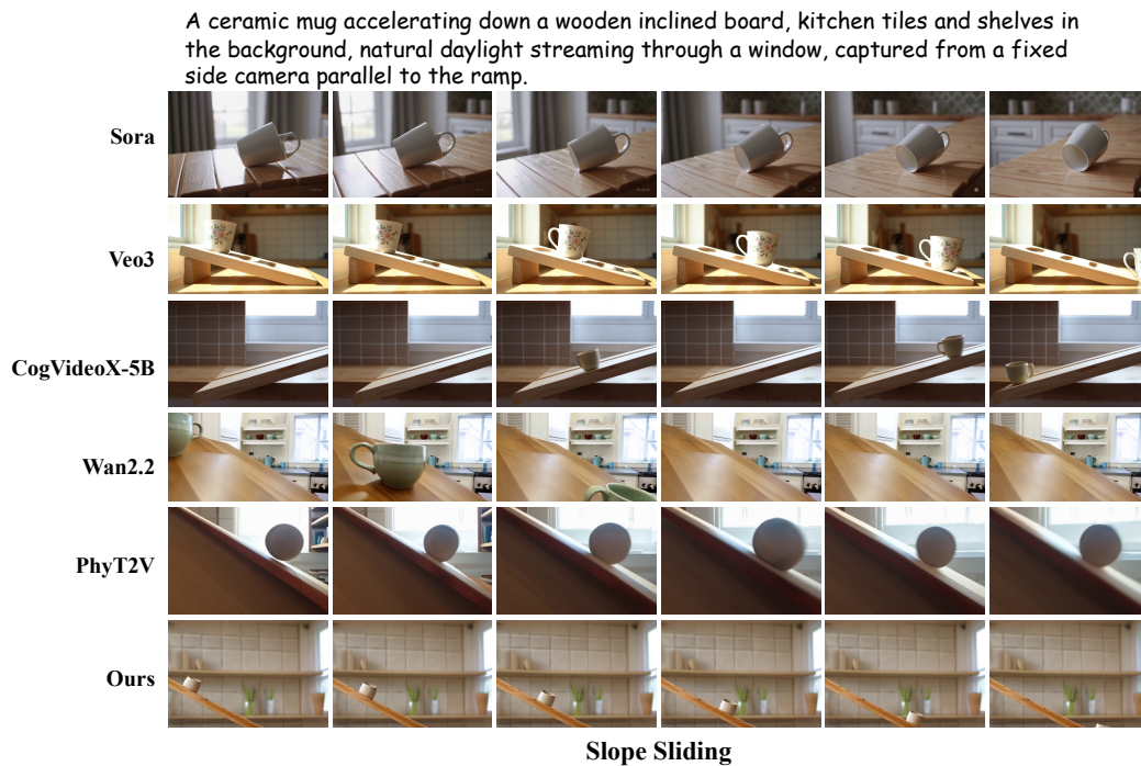
Figure 24: Visual comparisons on slope sliding.
