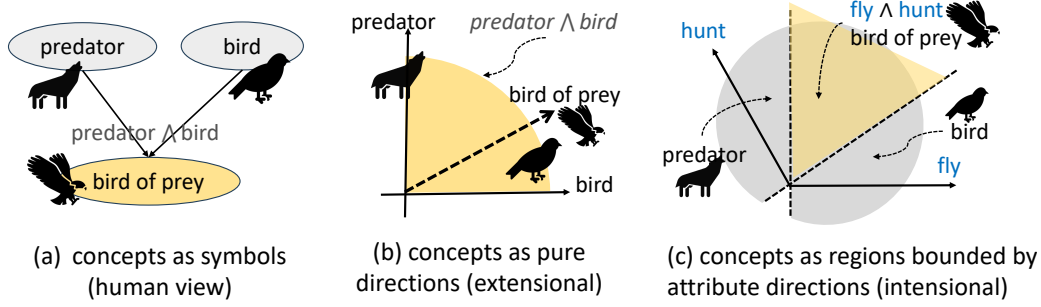
Figure 1: How LLMs encode conceptual structure. (a) Humans represent concepts as symbols and compose them using logical operators. (b) Under the standard extensional view, LLMs encode concepts as directions, where subsumption is interpreted through the relative orientation of vectors. (c) Under our intensional view, a concept is represented as the intersection of half-spaces defined by its attributes, and compositional semantics emerges through region intersection and union.
