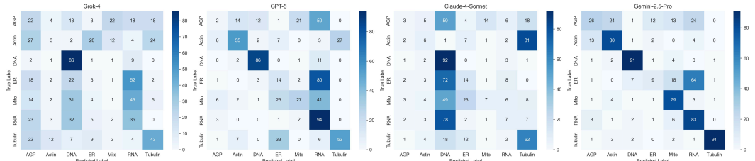
Figure 10: Confusion matrix on image channel task.
