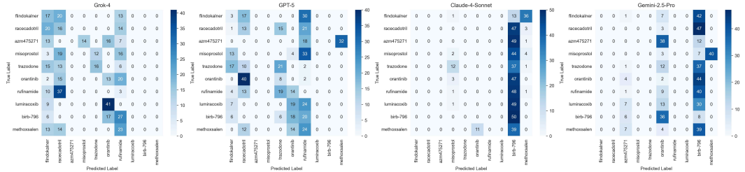
Figure 11: Confusion matrix on perturbation compound task.
