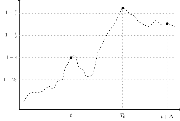
Figure 2: An example behavior of SGD for pure exploration in the learning phase (cf. Lemma 5). For appropriately chosen learning rates, if the correlation hits m_t \geq 1 - \varepsilon at time t , the SGD dynamics will enjoy the following behaviors with high probability: (i) the trajectory will never degrade too significantly, satisfying m_s \geq 1 - 2\varepsilon for all t \leq s \leq t + \Delta ; (ii) at some time s = T_0 \in [t, t + \Delta] , m_s improves to at least 1 - \frac{\varepsilon}{4} ; and (iii) thereafter, m_s may decrease, but will never fall below 1 - \frac{\varepsilon}{2} for all T_0 \leq s \leq t + \Delta .
