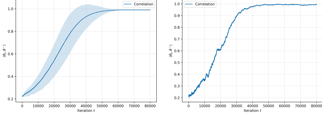
(a) Evolution of m_t = \langle \theta_t^*, \theta_t \rangle averaged across 100 runs. The shaded region plots one standard deviation.
