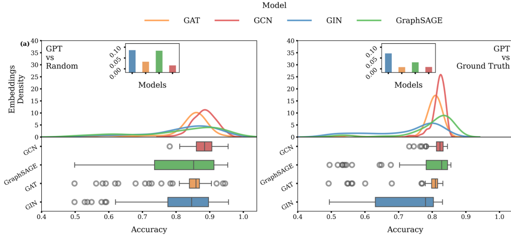
Figure 11: Distribution of final validation accuracy over the sweep of hyperparameters using different models on GPT-4o graphs using SPCETER embeddings Each panel summarizing the performance of four GNN architectures on validation set across our binary classification tasks using different seeds. The figures are related to the GNN results using embedding vectors. Within every panel, the top axis shows kernel-density estimates (KDEs) of per-run final accuracies, and the bottom axis shows each GNN architecture boxplots medians, interquartile ranges, whiskers, and outliers.
