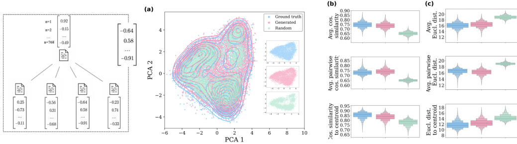
Figure 8: Embedding-space comparison for Claude graphs using SPECTER. Summing 768-d node embeddings to graph level, visualize the embedding space with 2D PCA (contours). Semantic comparison of citation graphs with Claude-generated references. As in the GPT-4o case, these results demonstrate that Claude retrieves topically appropriate references yet leaves a consistent semantic fingerprint that can be exploited for detection, in contrast to the near-indistinguishability at the purely structural level.
