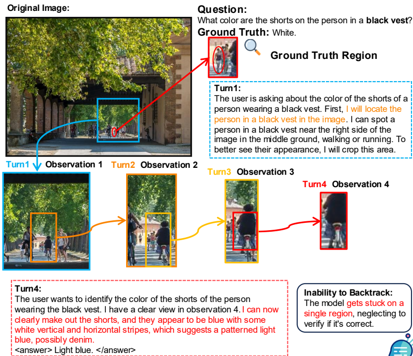
Figure 17: Failure case: Inability to Backtrack .
