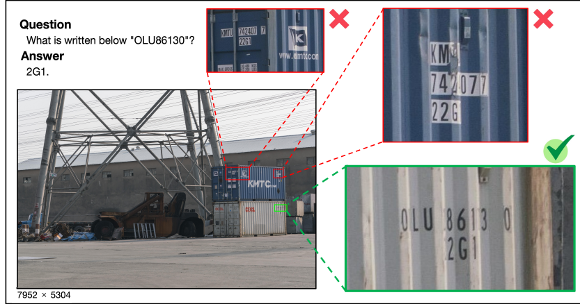
Figure 4: Illustration of the Visual Probe dataset. The Visual Probe dataset features 1) small targets; 2) disturbance objects; 3) high-resolution images. As a result, it is super challenging and requires iterative exploration and trial-and-error.
