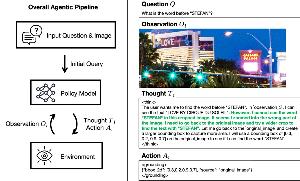
Figure 3: The overview of our framework for multi-turn agentic image tool use. During each turn, the model generates the thought and action iteratively based on the previous observation (or the input question and image). The observation at each turn is obtained based on the parameters indicated by the corresponding action.
