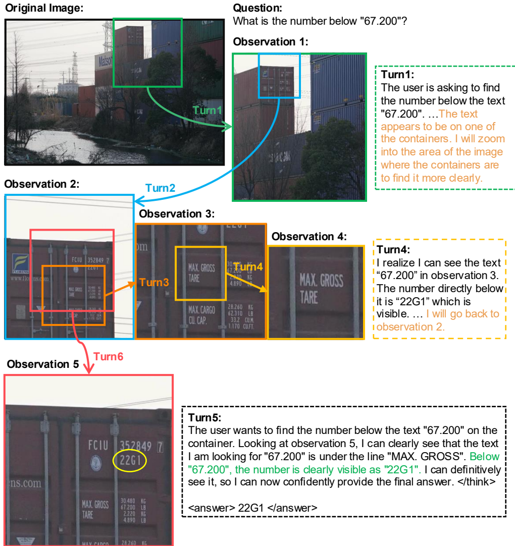
Figure 14: An example of visual search in a container yard generated by Mini-o3. The scene depicts stacked shipping containers with dense text markings. Our model performs multi-turn reasoning—targeted zoom-ins, cross-checking across observations, and corrective backtracking—to locate the string “67.200” and read the number directly beneath it. It outputs the correct value, “22G1”, demonstrating precise text localization and robust step-by-step verification in a cluttered setting.
