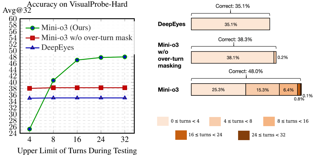
Figure 1: Left: Visual search accuracy continues to grow as the upper limit on the number of turns increases for Mini-o3. Right: Distribution of the correct trajectories under different numbers of interaction turns during testing. Mini-o3 demonstrates deeper thinking paths and stronger performance. Despite a small upper limit (i.e., 6 turns) during training, it shows the test-time turns scaling property: accuracy continues to grow as the maximum number of turns increases from 4 to 32.
