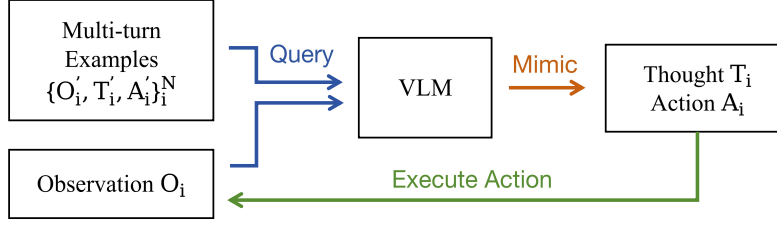
Figure 5: The pipeline of cold-start data collection.
