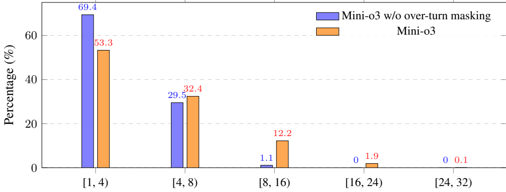
Figure 6: Distribution of interaction-turn percentages across five turn ranges during testing on VisualProbe-Hard. The percentages are calculated only on the correct responses.
