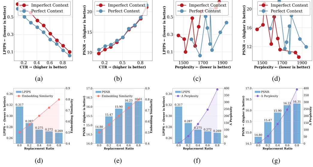
Figure 8: Detailed analysis of generator-tokenizer inconsistency. Results are evaluated with CTR ( \uparrow ), perplexity ( \downarrow ), PSNR ( \uparrow ), and LPIPS ( \downarrow ). (a–d): Exposure bias analysis—under the same CTR and lower perplexity, imperfect context yields higher LPIPS and lower PSNR. (e–g): Embedding unawareness analysis— \Delta Perplexity denotes the increase from original to replaced sequences; even with similar CTR and lower perplexity, original predictions can give worse PSNR/LPIPS, showing that higher-quality token sequences can be decoded into worse images.
