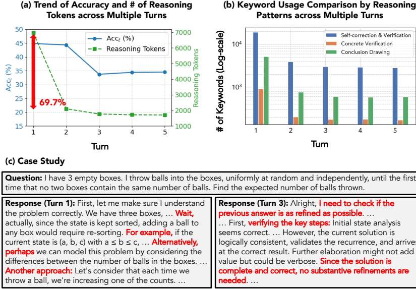
Figure 8: Reasoning behavior analysis of DeepSeek-R1.
