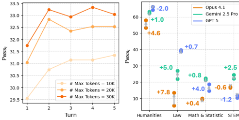
Figure 5: (Left) Performance over multiple turns for Gemini 2.5 Pro; (Right) Domain analysis for flagship reasoning LMs.
