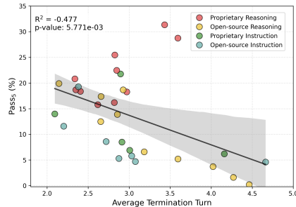
Figure 7: Correlation between the average termination turn ratio and \text{PASS}_5 .
