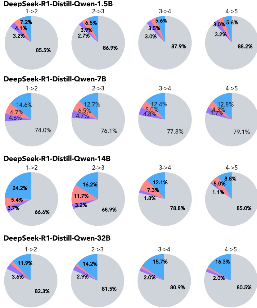
Figure 13: Transition analysis of the self-refinement capability of four different reasoning models: DeepSeek-R1-Distill-Qwen- \{1.5, 7, 14, 32\} B.
