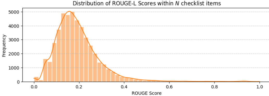
Figure 9: Diversity of N checklist items.
