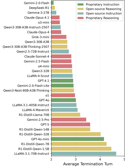
Figure 6: Average termination turn ratio in self-refinement across 32 instruction-tuned and reasoning models.
