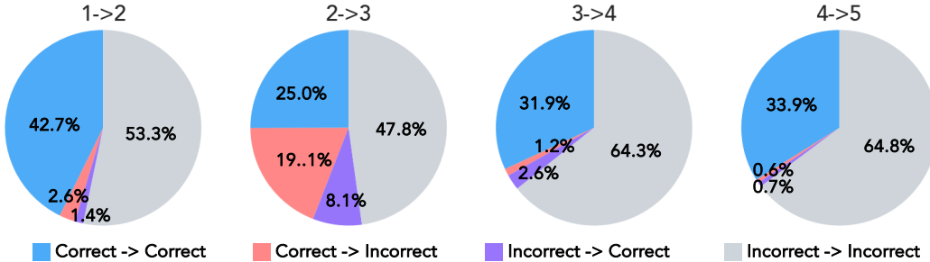
Figure 12: Transition analysis of the self-refinement capability of DeepSeek-R1 on REFINEBENCH under the self-refinement setting.
