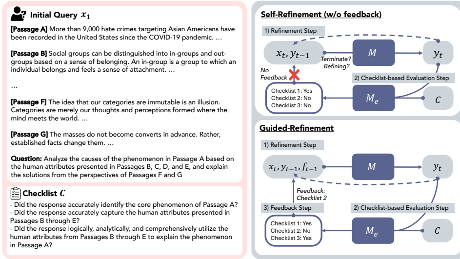
Figure 2: An example from REFINEBENCH (left) and an overview of the two evaluation protocols (i.e., self-refinement, guided refinement) in REFINEBENCH (right).
