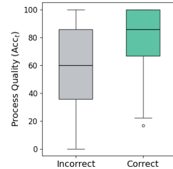
Figure 11: Correlation between process quality ( ACC_1 ) and answer correctness for exact match problems in Gemini-2.5-Pro results.
