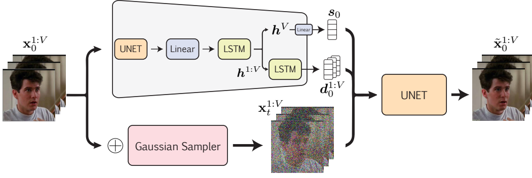
Figure 1: DiffSDA processes sequences \mathbf{x}_0^{1:V} via semantic and stochastic encoders (top and bottom). Their outputs (s_0, d_0^{1:V}, \mathbf{x}_t^{1:V}) are fed to a stochastic decoder yielding a denoised \tilde{\mathbf{x}}_0^{1:V} (right).
