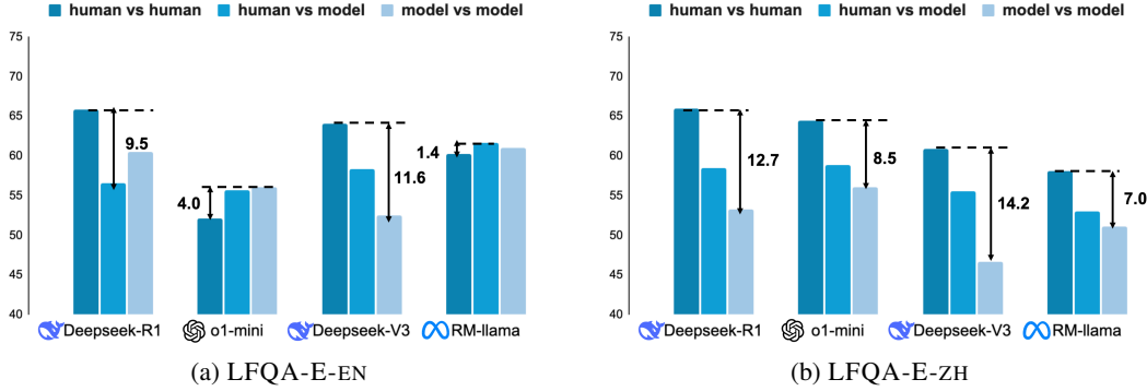
Figure 2: Performance of different models on our three settings on LFQA-E.
