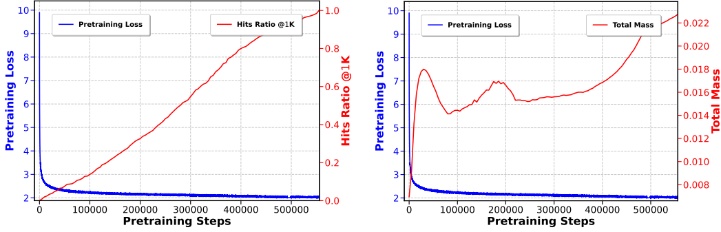
(a) Top 1K jet bi-gram hit ratios w.r.t. the final step.
