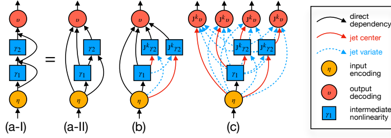
Figure 3: Carving a two-block net. (a) Nested entanglements. (b) Inner expansion at \gamma_2 . (c) Outer expansion at Dec, yielding 4 explicit paths. Interpreting a model component entails selection. Jet centers trace paths through modules of interest; jet variates trace paths through those excluded from that focus.
