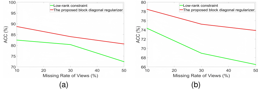
Figure 4: Clustering accuracies (ACC, %) of the proposed method and the conventional low-rank constraint model on the COIL-20 and noisy COIL-20 databases with different missing rates, respectively.
