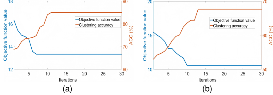
Figure 3: Objective function value and clustering accuracy of the proposed method versus the number of iterations on the (a) BBCSport and (b) BUAA databases, respectively.
