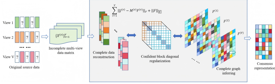
Figure 1: The flowchart of the proposed CBDS_IMVC method.
