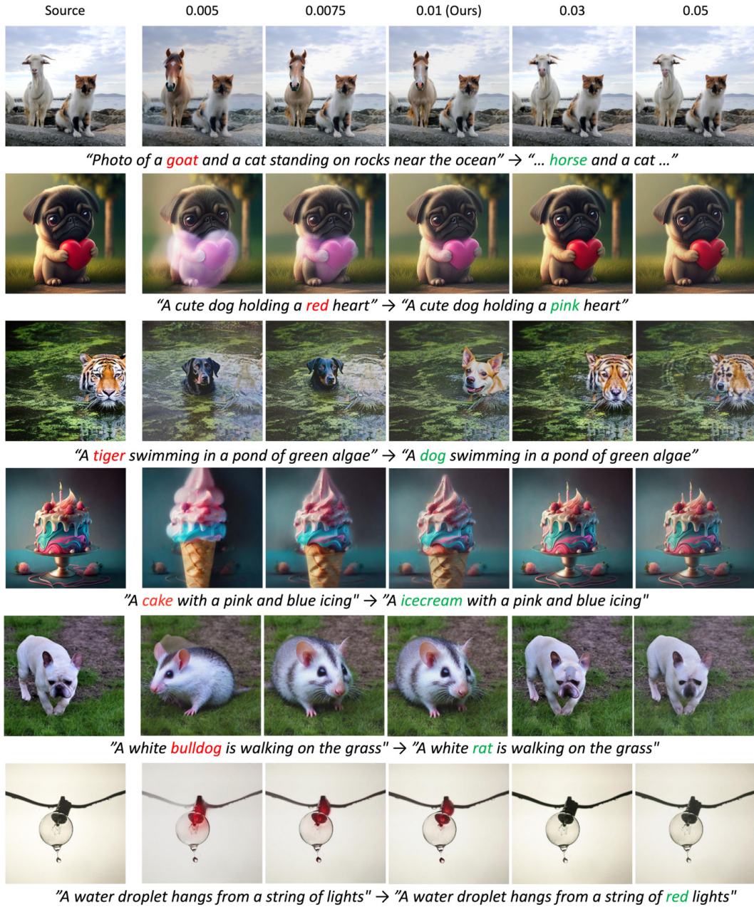
Figure 12: Ablation results for \zeta .
