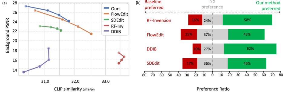
Figure 3: Quantitative and human preference evaluation. (a) Trade-off between CLIP similarity versus background PSNR. The darker the blob, the larger CFG scale. (b) User preference results. Each bar shows the proportion of responses favoring the baseline (red), showing no preference (gray), or favoring our method (green). Bars are centered at 0 to emphasize directional preference. Across all comparisons, our method is preferred.
