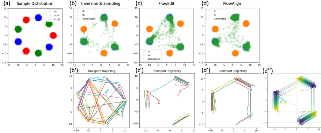
Figure 9: Results of inversion-based transformation, FlowEdit and FlowAlign on 2D toy dataset.
