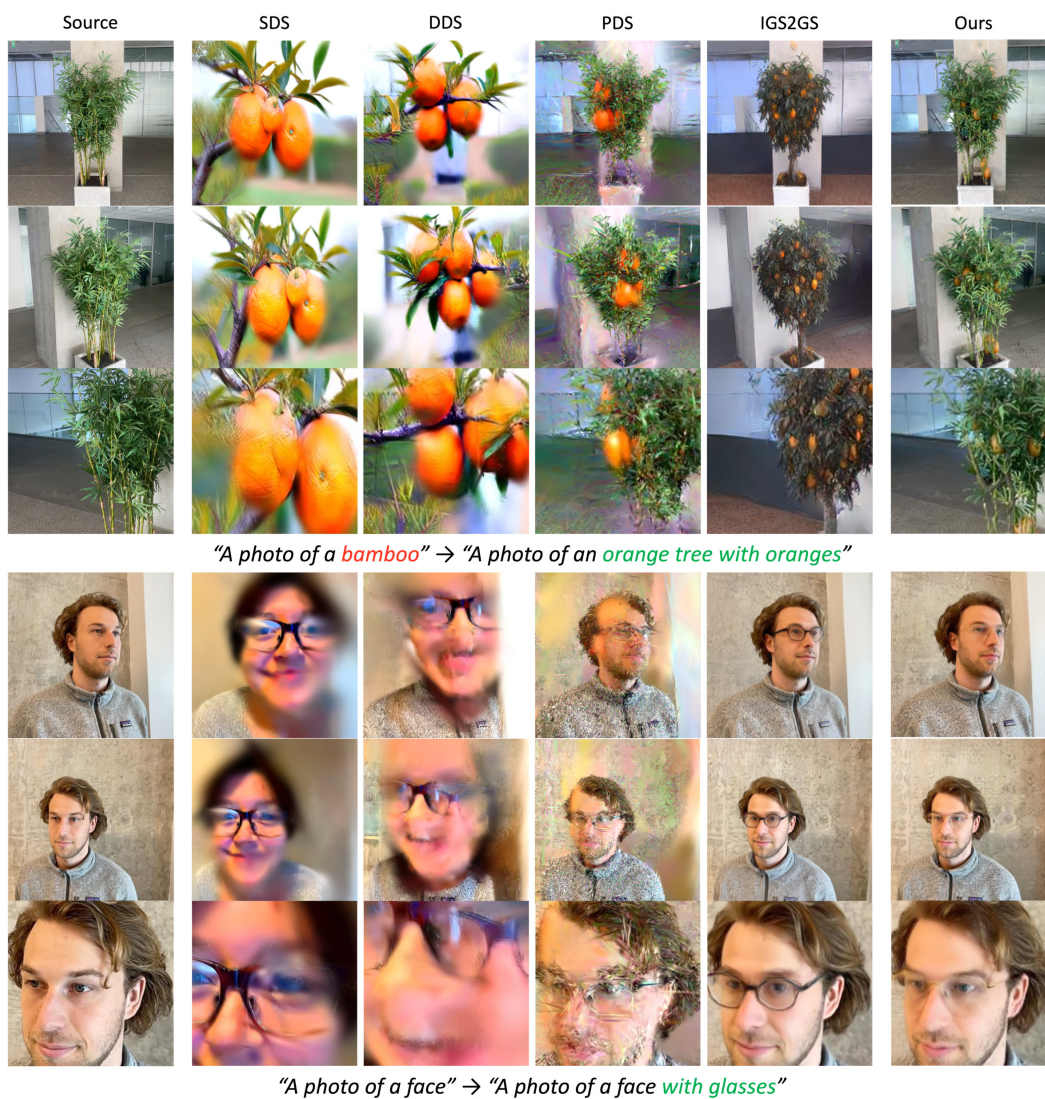
Figure 17: Additional results for 3D editing.
