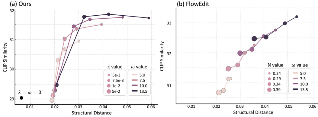
Figure 13: Ablation study for hyperparameters of FlowAlign and FlowEdit.
