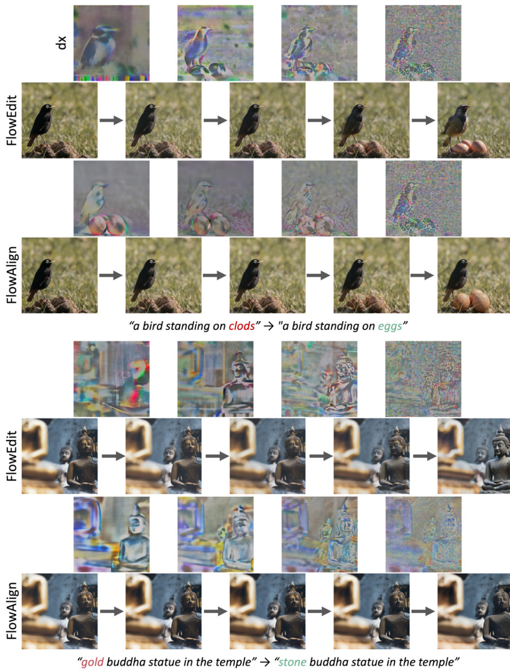
Figure 21: Visualization of FlowEdit and FlowAlign editing trajectories.
