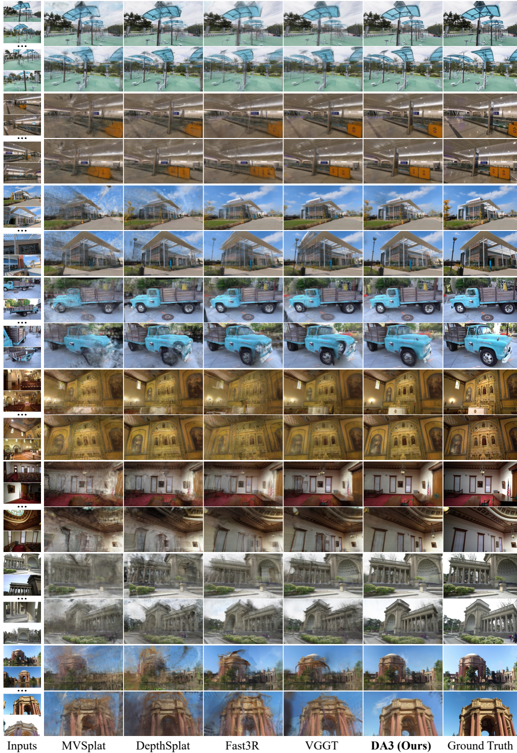
Figure 9: Qualitative comparisons with state-of-the-art methods for visual rendering. The first column shows the selected input views, while the remaining columns display novel views rendered by comparison models and ground truth. For each scene, two rendered novel viewpoints are presented in consecutive rows. The first three scenes are from DL3DV, the following two are from Tanks and Temples, and the last three are from MegaDepth. Compared to other methods, our model consistently achieves superior rendering quality across diverse and challenging scenes.
